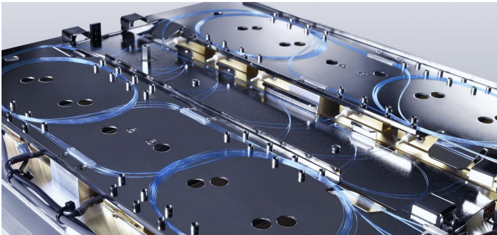
Fig. 12: Fibre laser
